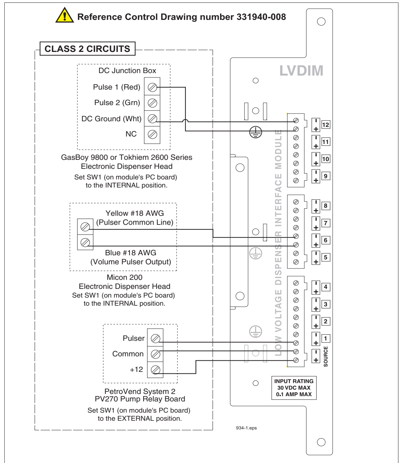
Figure 19. LVDIM Module POS/Pulser Connections
