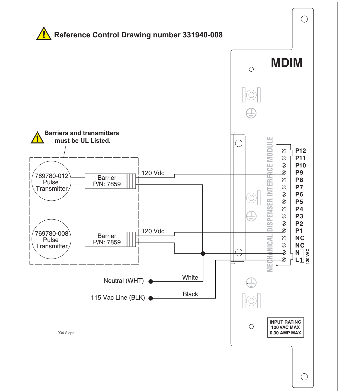
Figure 18. MDIM Module Pulser Connections
