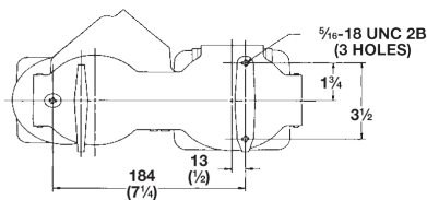
Bottom View All Configurations
