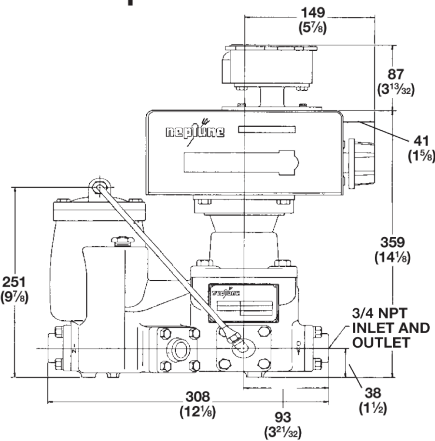
1" 4D-MD with 600 Series Register and pulser
