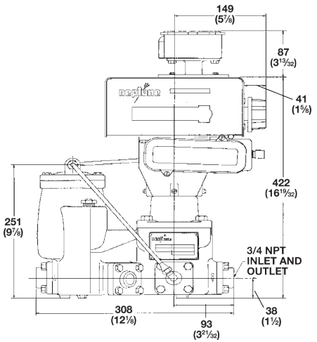
1" 4D-MD with 600 Series Register, pulser, and ATC
