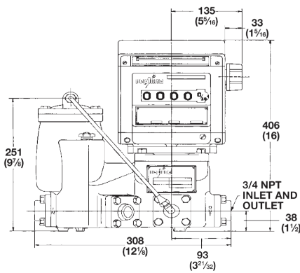
1" 4D-MD with 800 Series Register
